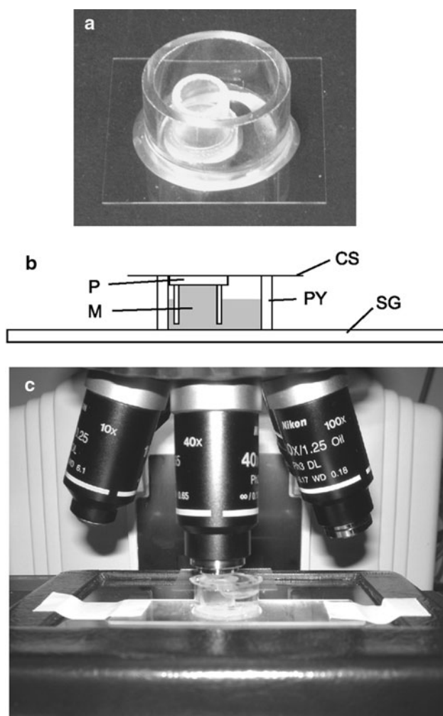
Fig. 1 Anaerobic thermophile observation chamber (ATOC). An intermediate construction of ATOC (a), a schematic illustration of completed ATOC (b), and an ATOC placed on a Microheat plate, which was set below an objective (c). CS coverslip, M medium, P partition, PY Pyrex piece, SG slide glass
